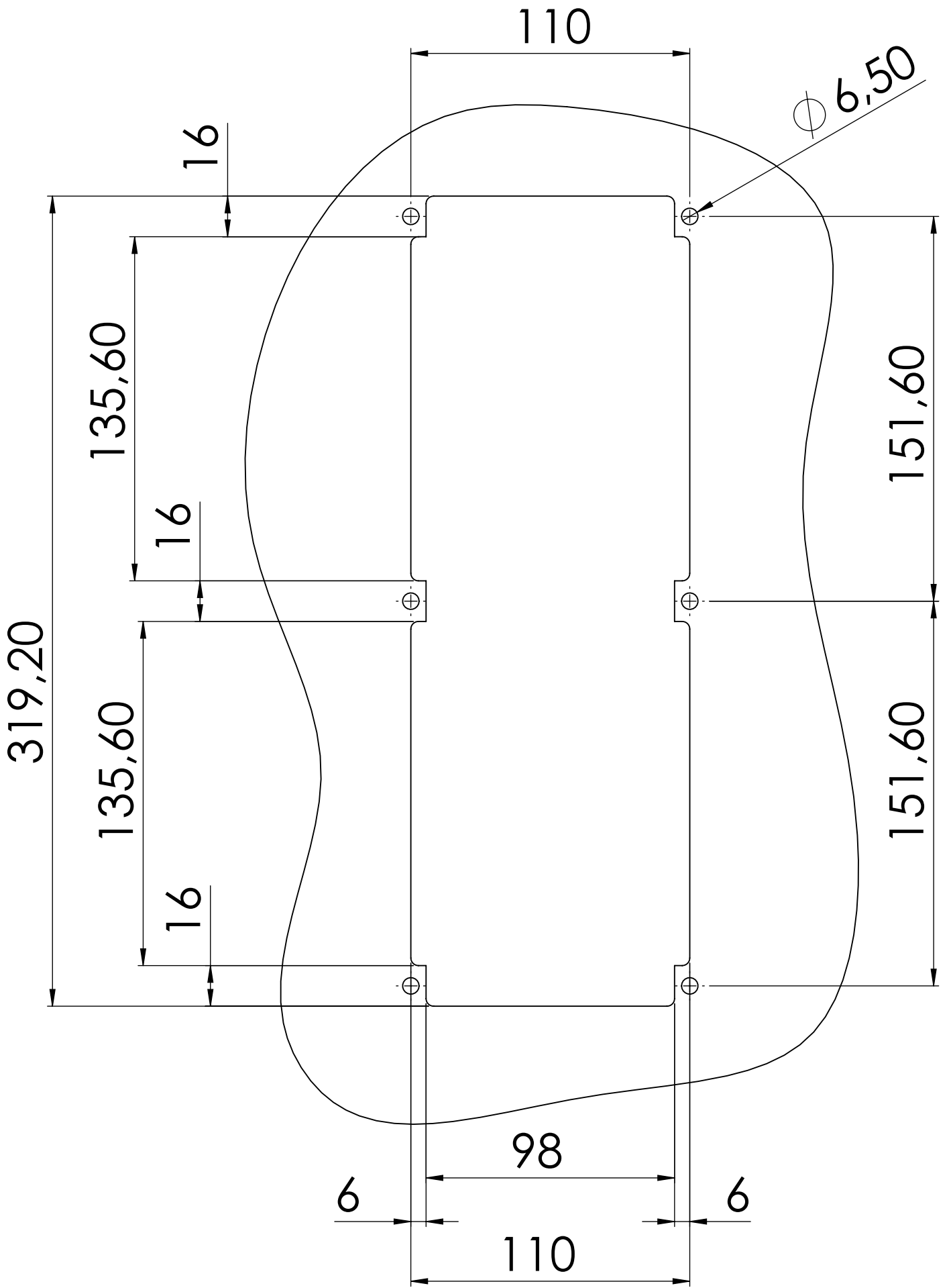
cutting drawing for intercom VENDONE
